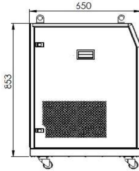
RIGHT VIEW
